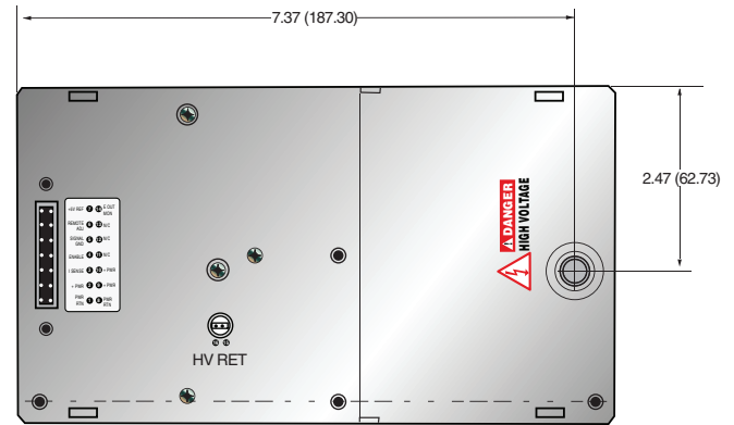
TOP VIEW UMW 20KV
